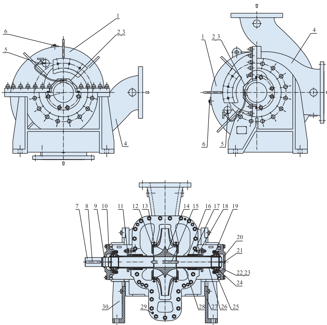
HSC Structural drawing of model HSC-L type horizontal pump
