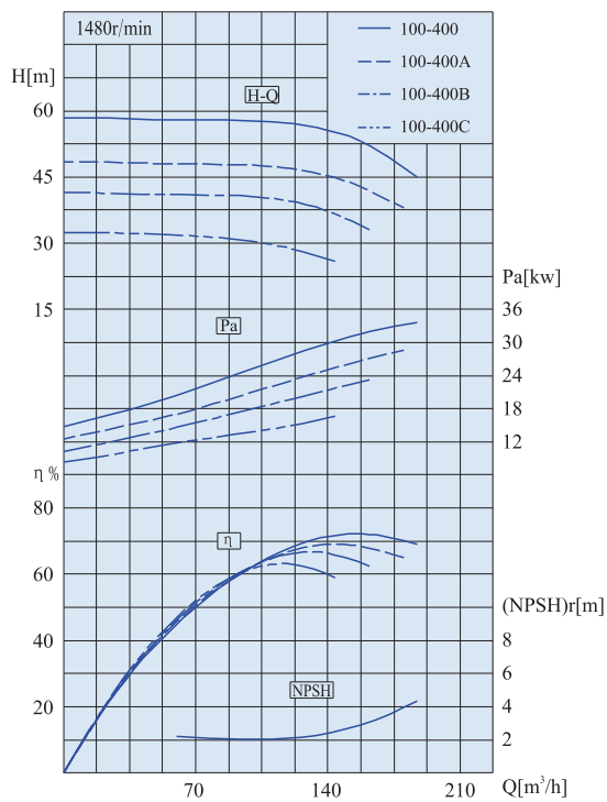
HSC/HVC type pump performance curve chart
