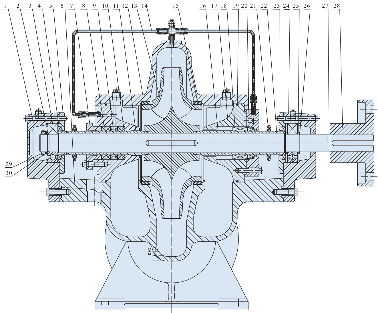
HSC Structural drawing of model HSC horizontal pump
