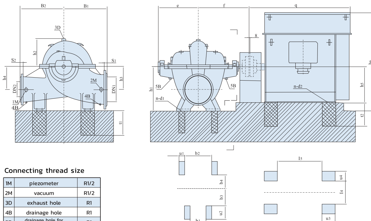
Pump basic
