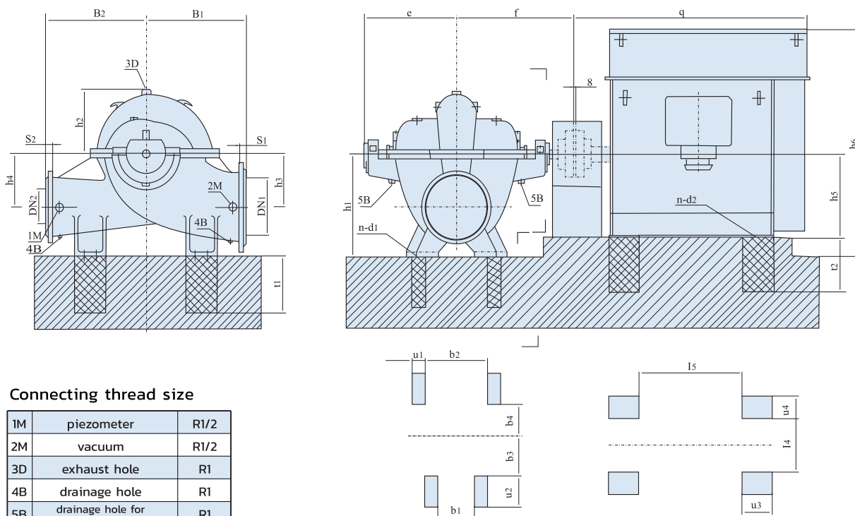
Pump basic
